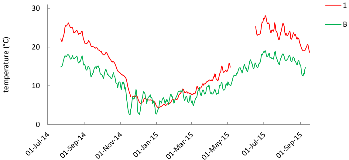
Figure 5 Average daily temperatures measured in Bings Creek (green line) versus temperature recorded at a 1m depth (red line) in Somenos Lake, July 2014-September 2015.
