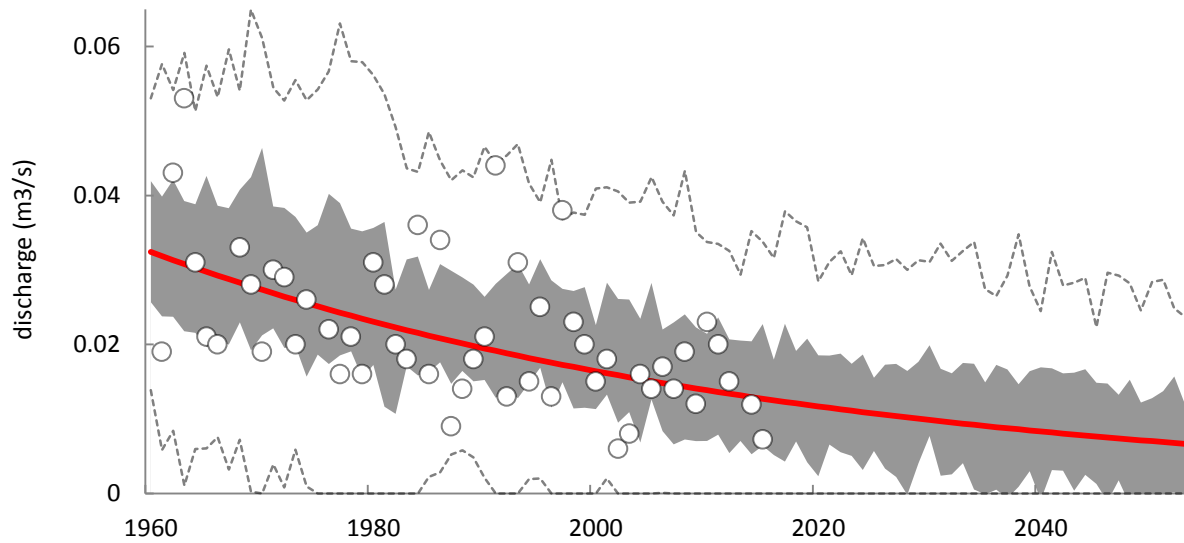
Figure 2: Mean August discharge (circles) in Bings Creek, 1960-2015 (Environment Canada data from wateroffice.ec.gc.ca/ ). The red line shows modelled mean August discharge with a logistic regression fitted to historic data. This model was used to generate hindcasts and forecasts of mean August discharge from 1960 to 2050 by modelling potential annual variability as a function of the difference between observed discharge data and modelled hindcast data. The gray line shows the \pm 50\% confidence interval and the dotted lines show the \pm 95\% confidence intervals after 100 simulations.
