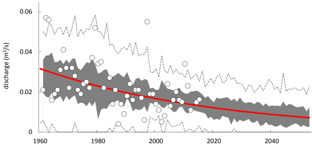
Figure 3: Mean September discharge (circles) in Bings Creek, 1960-2015 (Environment Canada data from wateroffice.ec.gc.ca/ ). The red line shows modelled mean September discharge with a logistic regression fitted to historic data. This model was used to generate hindcasts and forecasts of mean September discharge from 1960 to 2050 by modelling potential annual variability as a function of the difference between observed discharge data and modelled hindcast data. The gray line shows the \pm 50\% confidence interval and the dotted lines show the \pm 95\% confidence intervals after 100 simulations.
