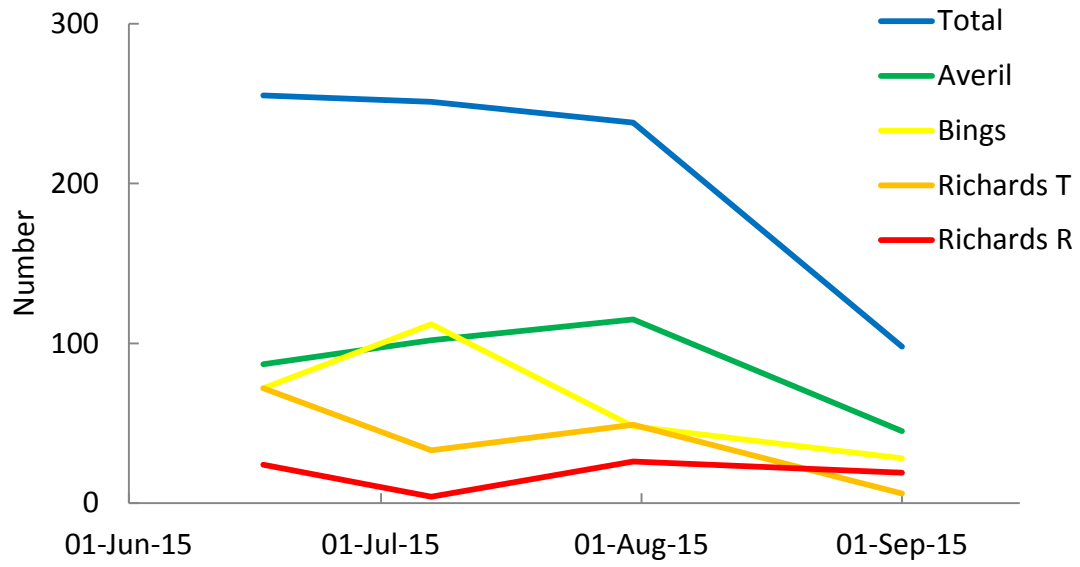
Figure 10: Trends in catches of Coho Salmon at each of the four creek sampling sites during the summer of 2015)
