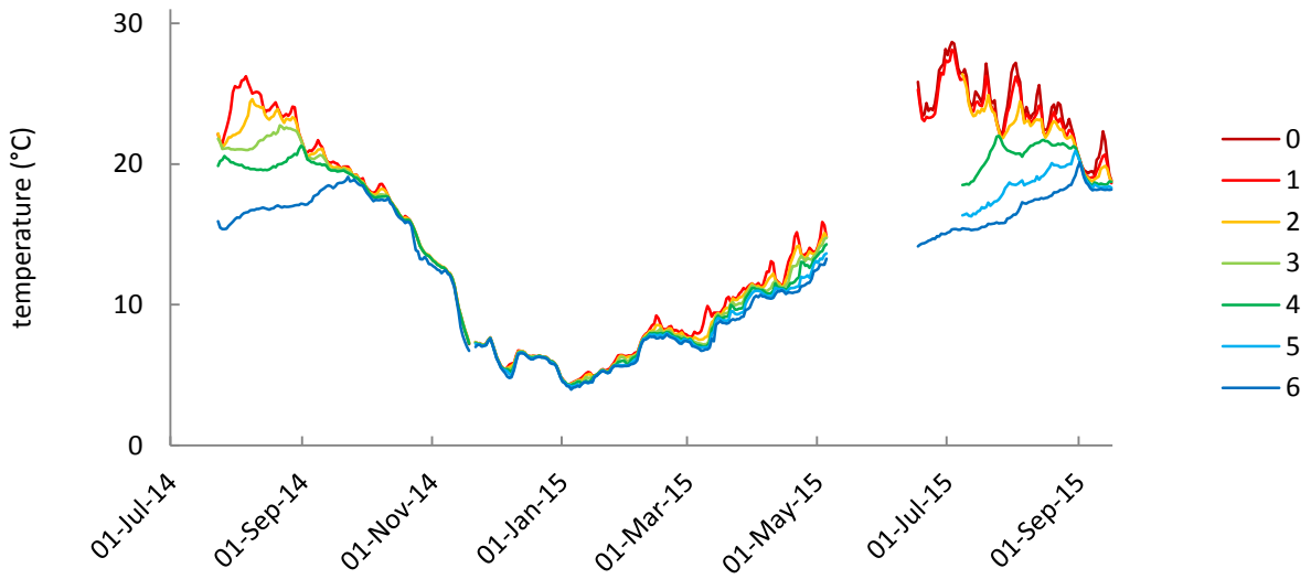
Figure 4: Average daily temperatures measured at the Somenos Lake station, July 2014-September, 2015 at 0m (surface) to 6m depth. Note the missing data for early May to mid-June due to the disappearance of the temperature data logger array.
